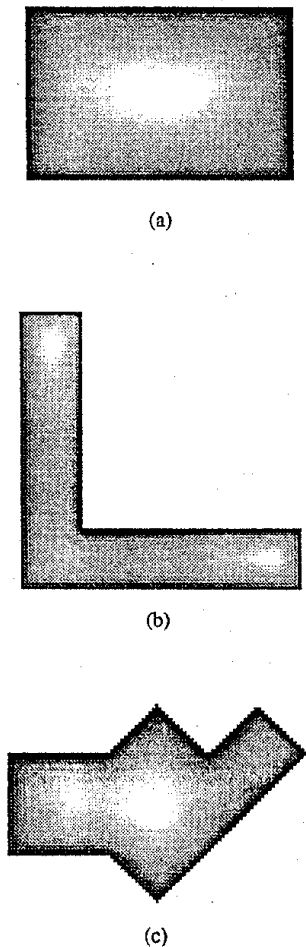
Fig. 3. Newtonian potential within (a) a rectangle; (b) an "L"-shaped object; and (c) the object used in Fig. 19 of [20]. The brighter a point, the lower is the potential. The brightness is made to vary logarithmically with potential value.
