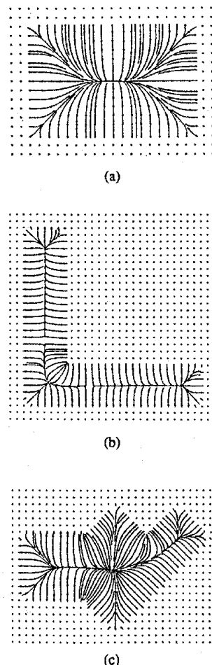
Fig. 4. Streamline representations of Newtonian force fields within regions shown in Fig. 3.
